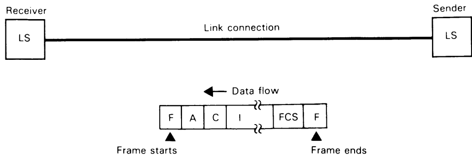
Figure 11. SDLC Transmission Frame
