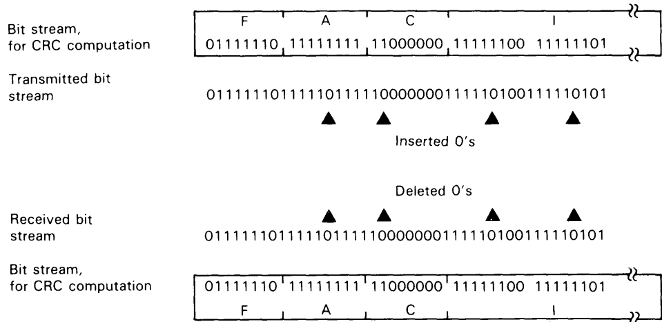
Figure 15. Zero Insertion and Deletion
