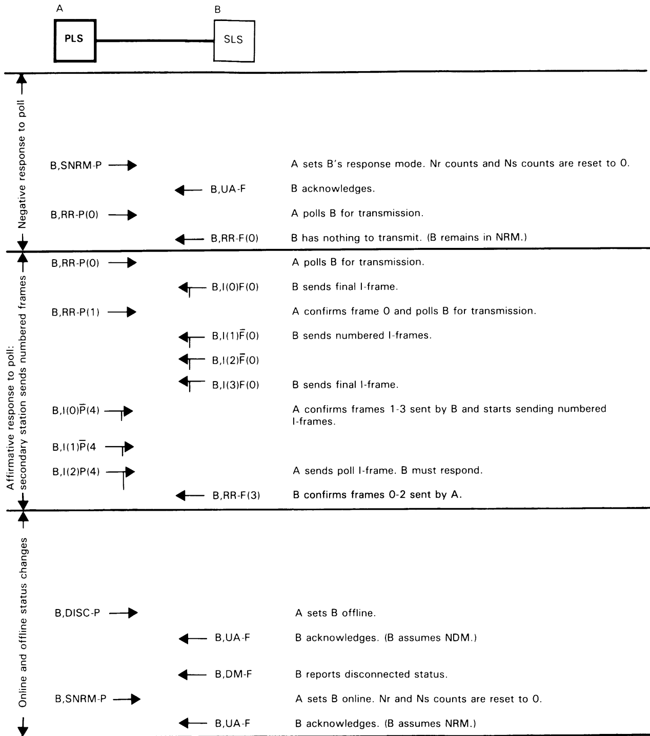
Figure 24 (Part 1 of 2). Two-way Alternate Exchanges on Nonswitched Point-to-Point Links
