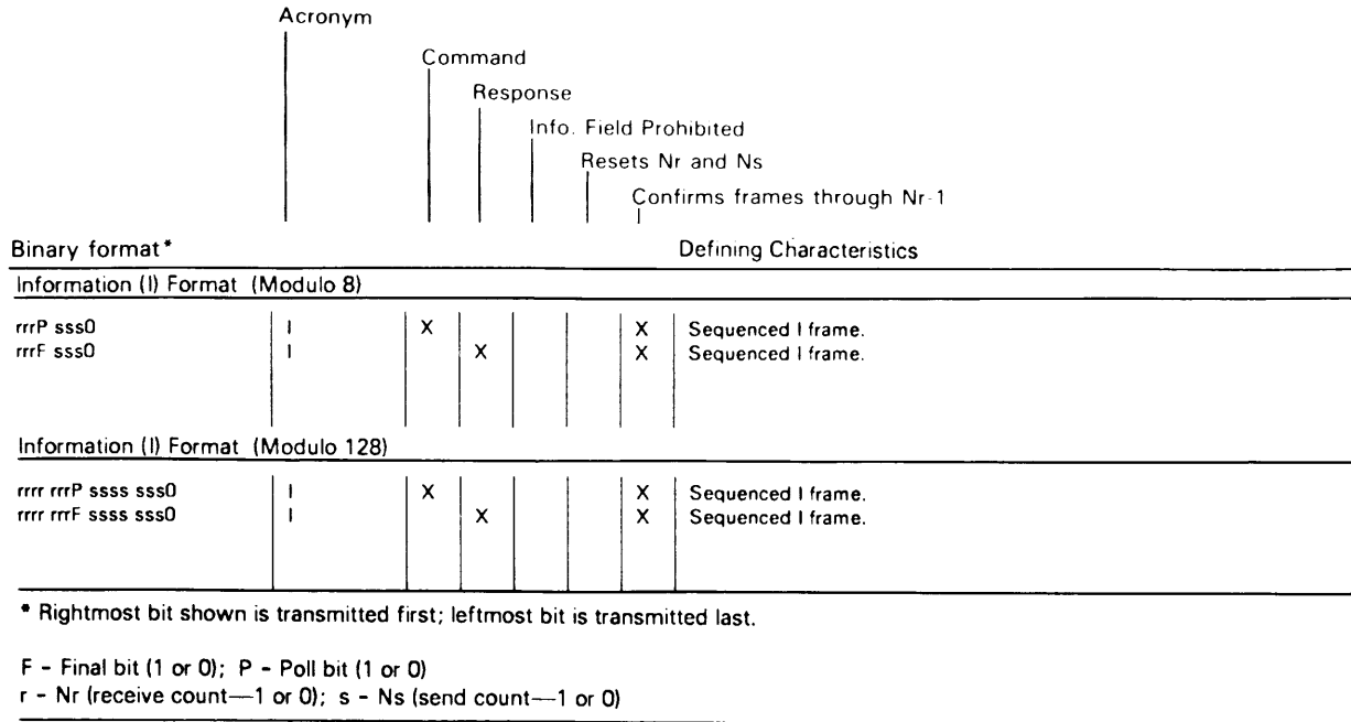
Figure 18 (Part 2 of 2). Summary of Command and Response C Fields
