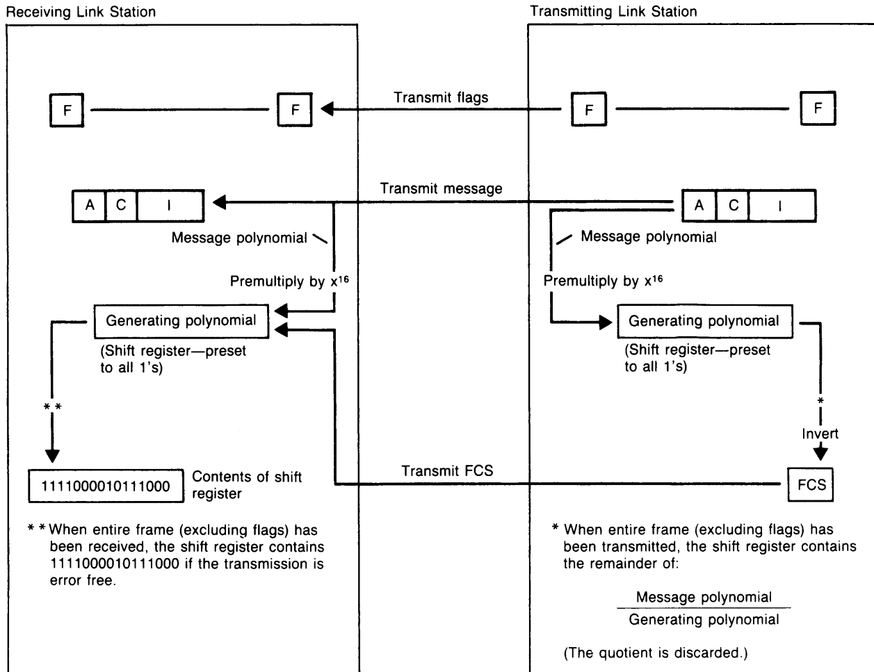
Figure 31. CRC Operation with SDLC
