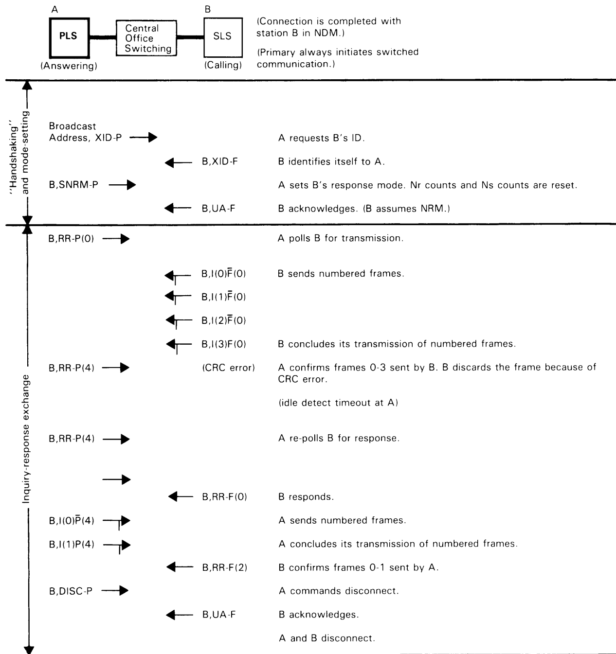
Figure 27. Two-way Alternate Exchanges on Switched Point-to-Point Links
