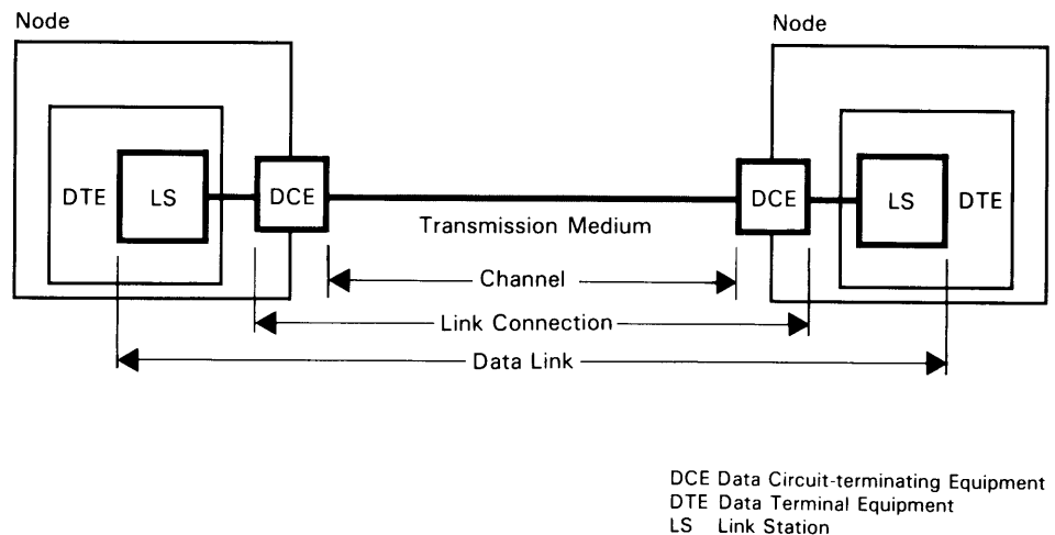
Figure 1. Components of a Data Link
