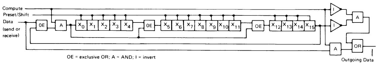
Figure 30. An Example of Cyclic Redundancy Checking
