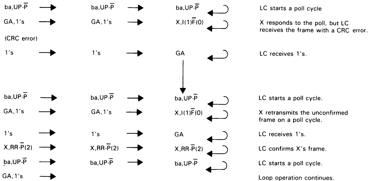
Figure 28 (Part 2 of 2). Two-Way Alternate Exchanges on SDLC Loops
