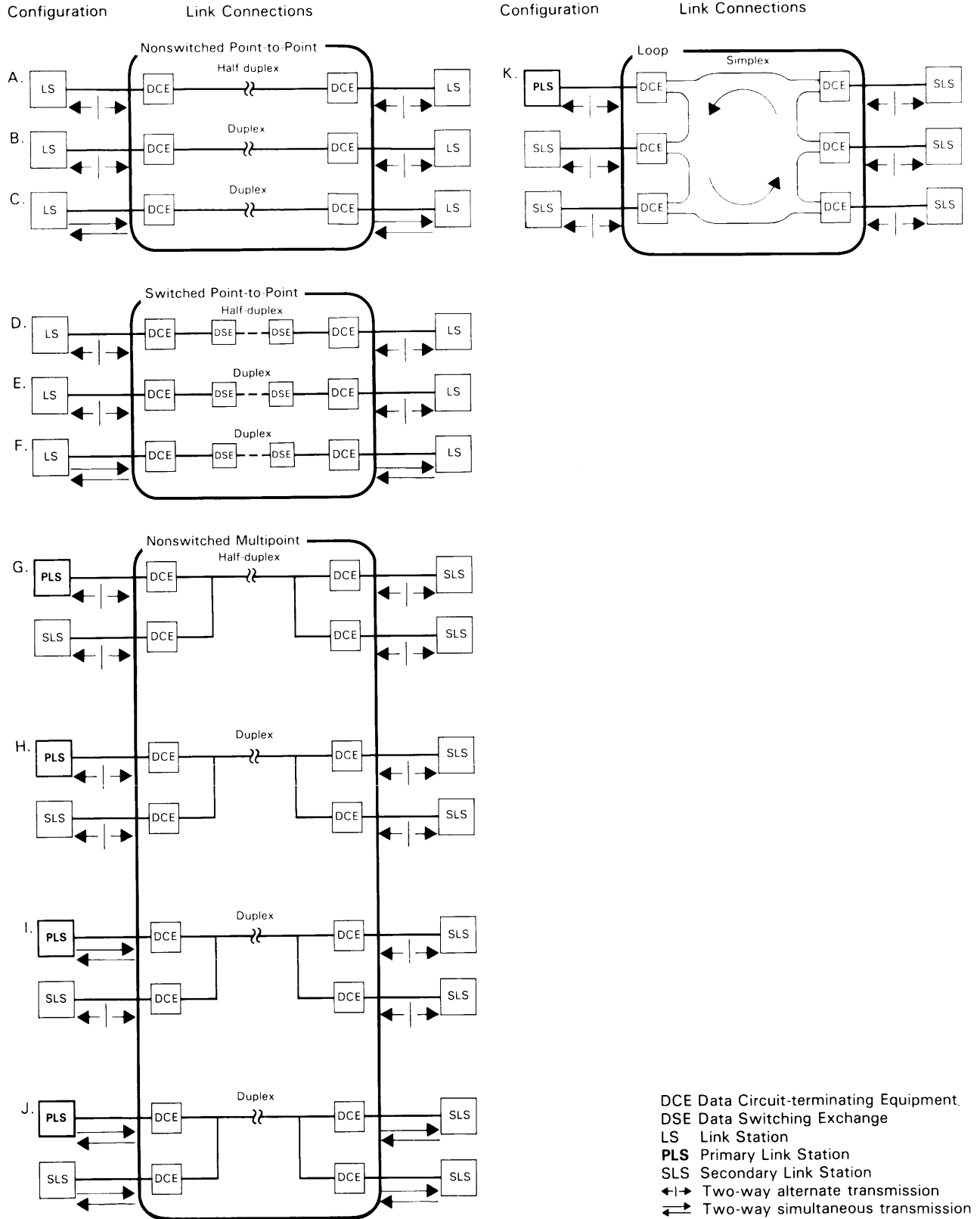
Figure 4. Link Connection Configurations and Link Station Operation
