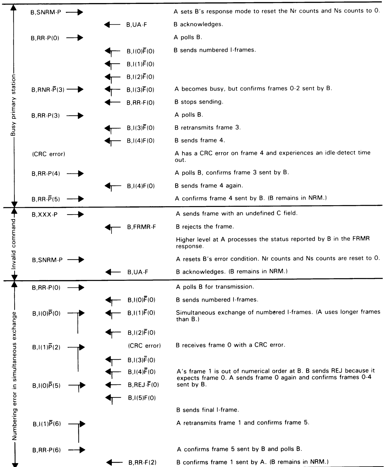
Figure 25 (Part 2 of 2). Two-way Simultaneous Exchanges on Nonswitched Point-to-Point Links
