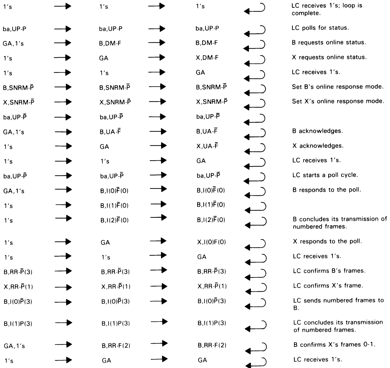
Figure 28 (Part 1 of 2). Two-Way Alternate Exchanges on SDLC Loops
