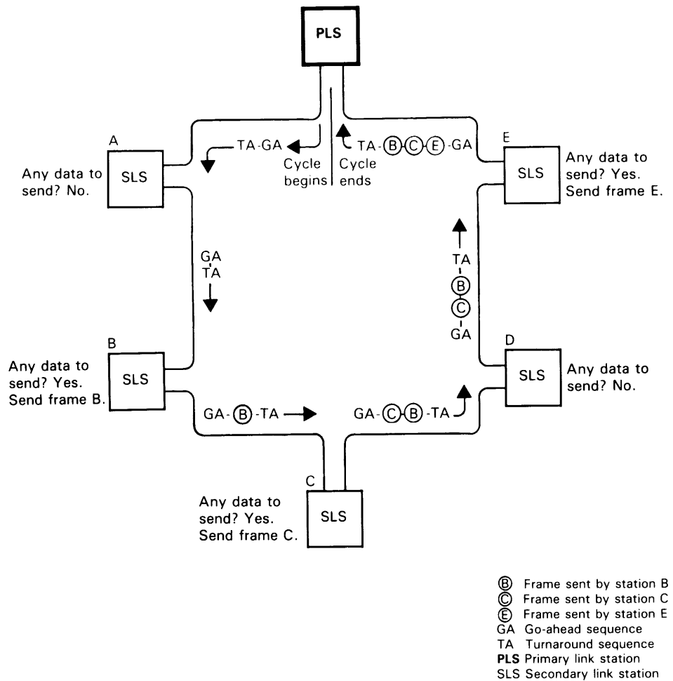
Figure 22. SDLC Loop Exchanges: Secondary Stations Transmitting
