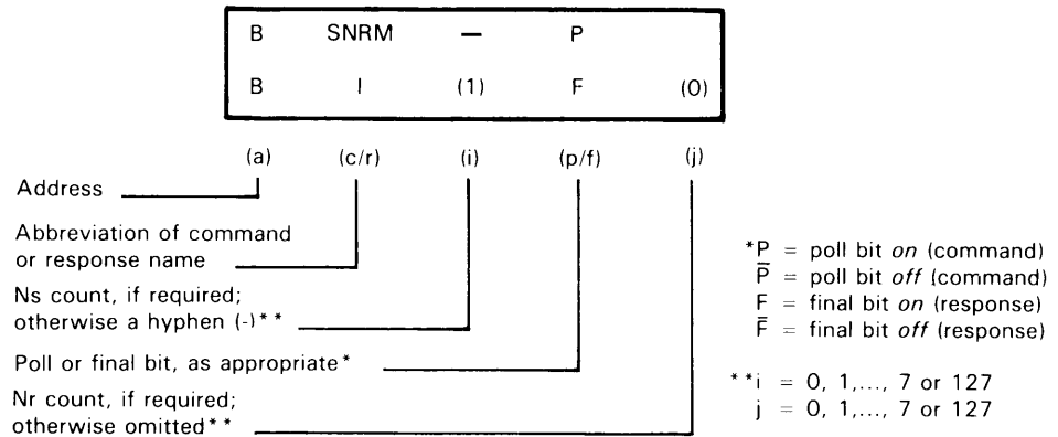
Figure 23. Format of Examples of SDLC Exchanges
