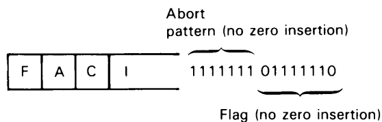
Figure 17. Transmitting Station Aborts Transmission
