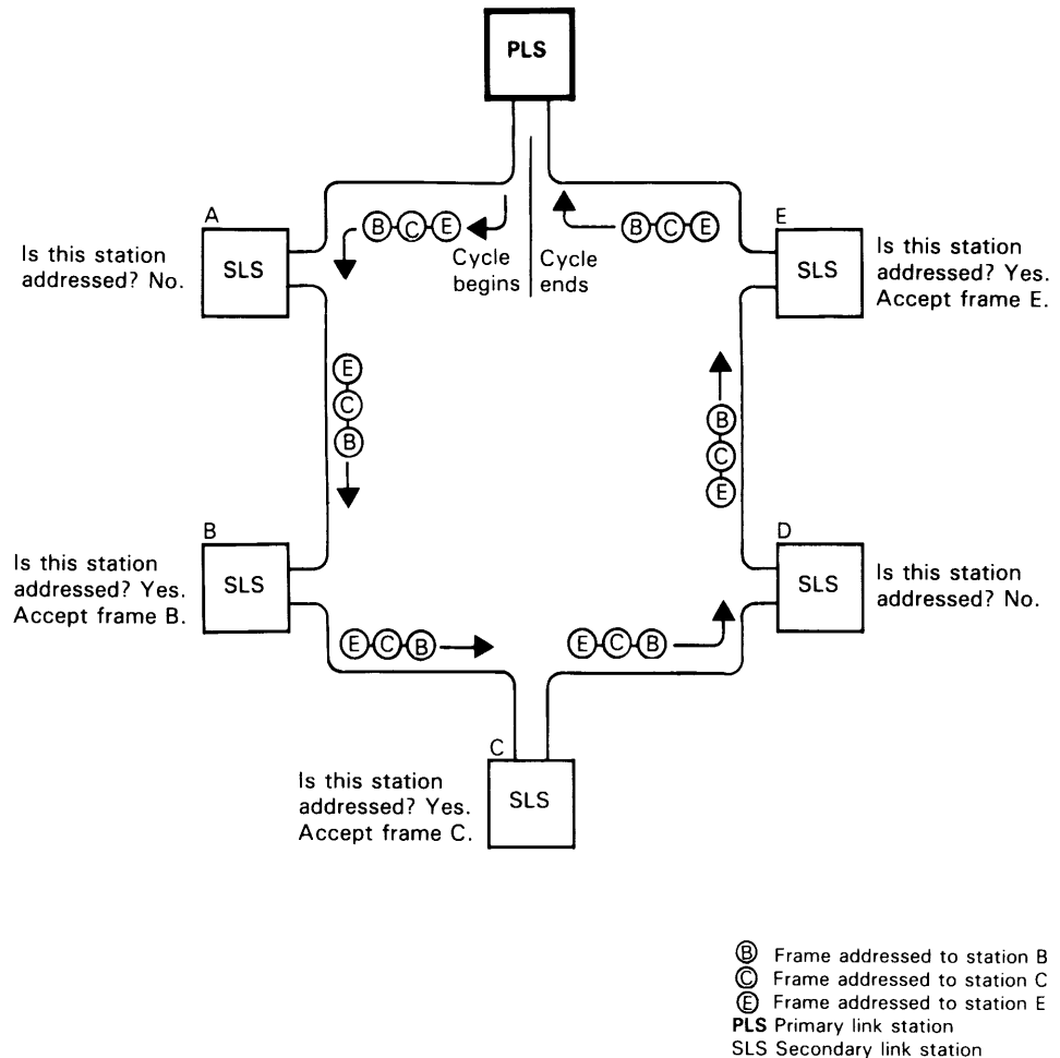
Figure 21. SDLC Loop Exchanges: Primary Station Transmitting
