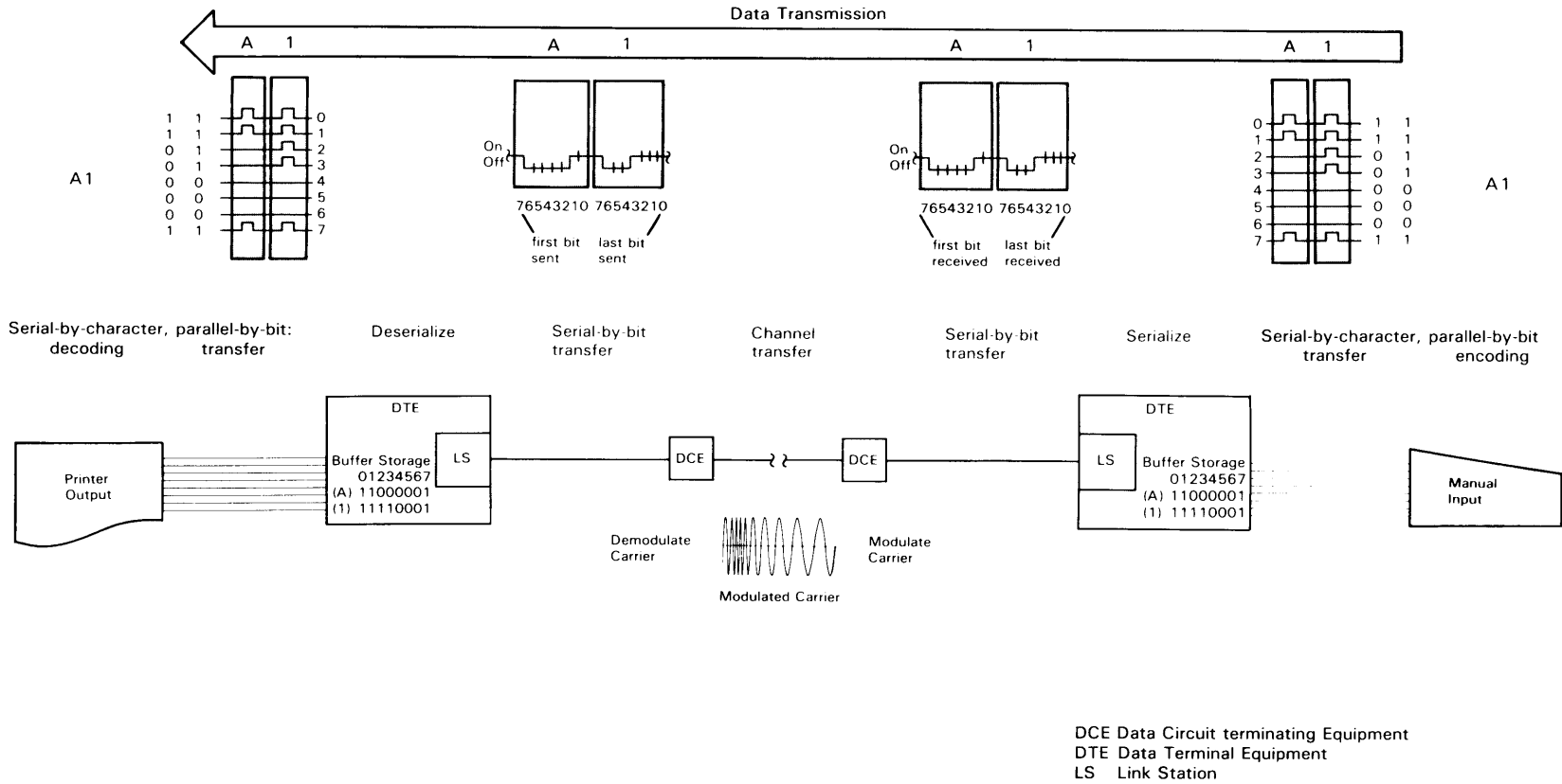
Figure 5. Data Conversion for Data Link Transfer
