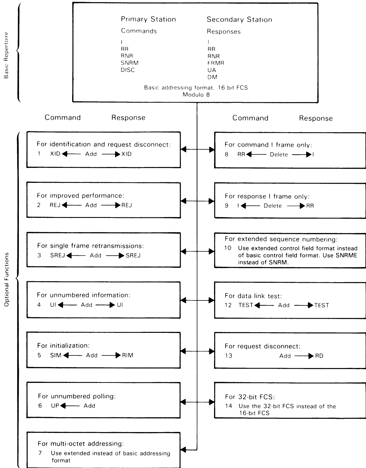
Figure 32. HDLC Unbalanced Normal Class of Procedures
