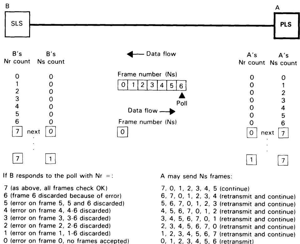
Figure 14. Example of Modulo-8 Frame Numbering
