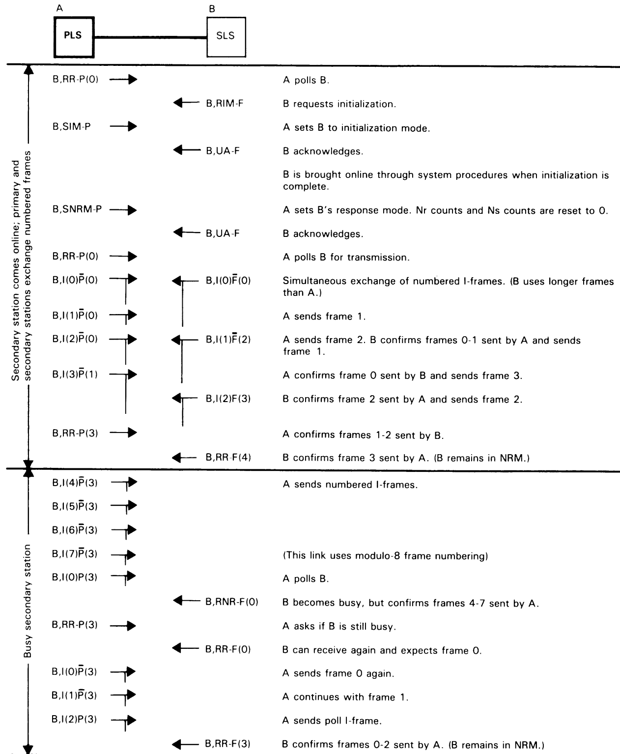
Figure 25 (Part 1 of 2). Two-way Simultaneous Exchanges on Nonswitched Point-to-Point Links
