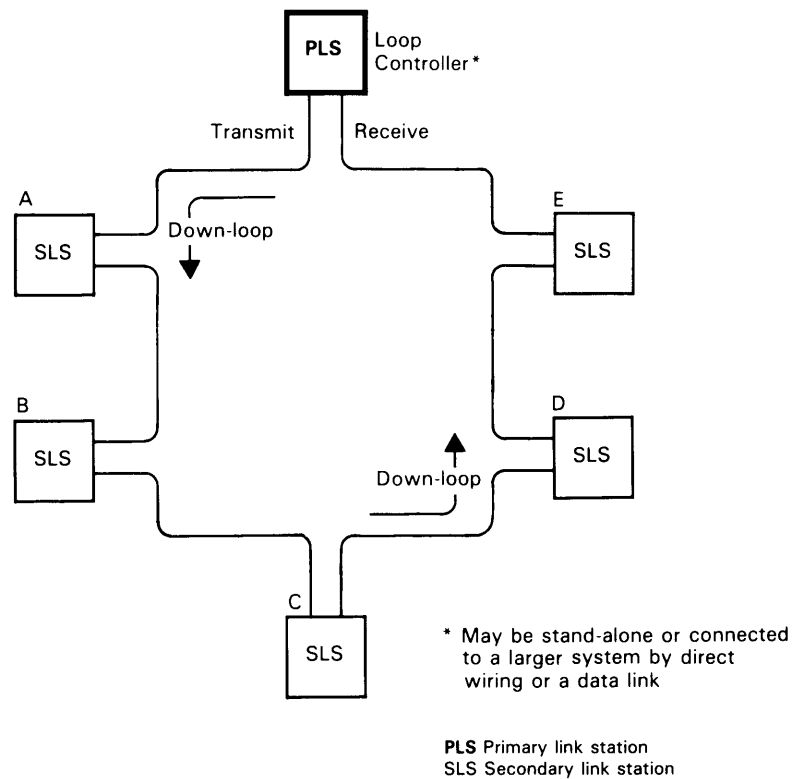
Figure 20. Loop Configuration
