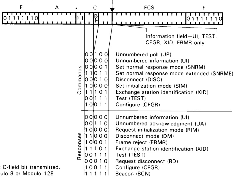
Figure 29. SDLC Frames, As Transmitted
