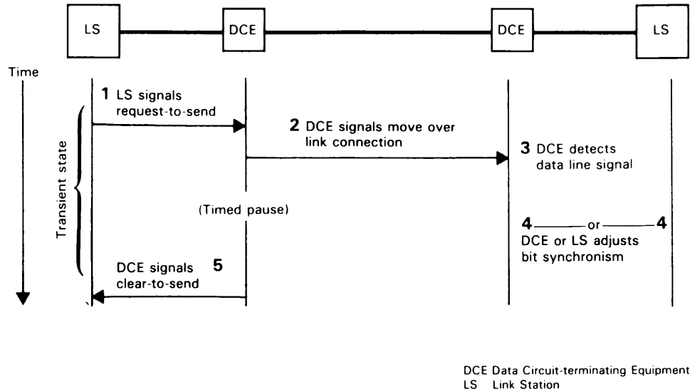
Figure 9. Period of the Transient State
