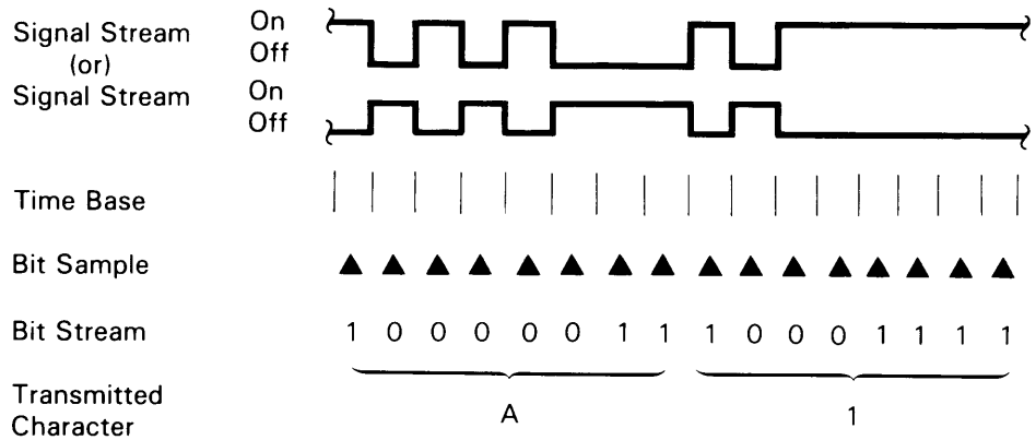
Figure 8. Invert-on-Zero Transmission Coding
