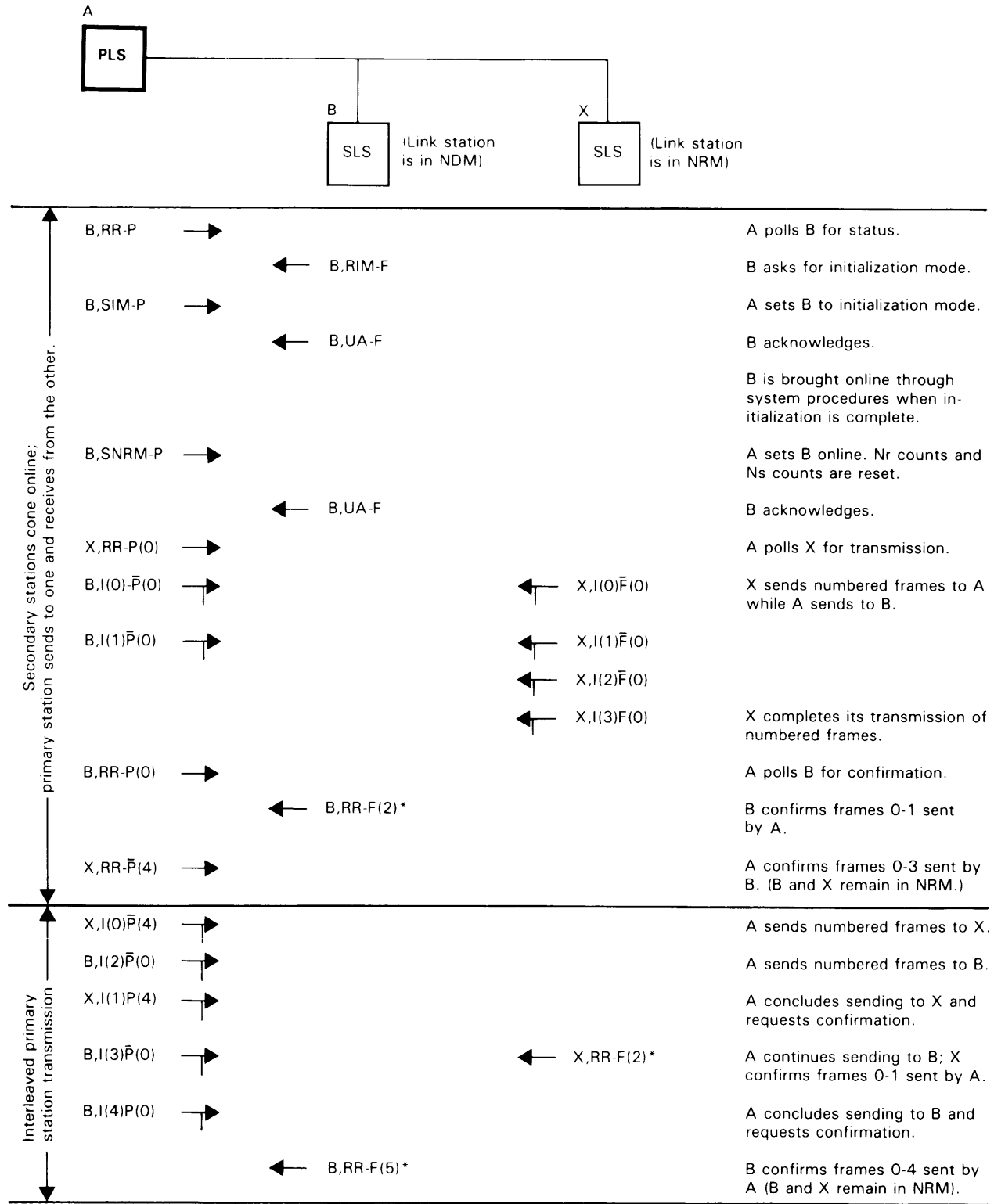
Figure 26. Two-way Simultaneous Exchanges on Nonswitched Multipoint Links
