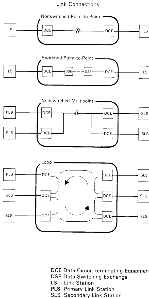
Figure 3. Link Connection Configurations
