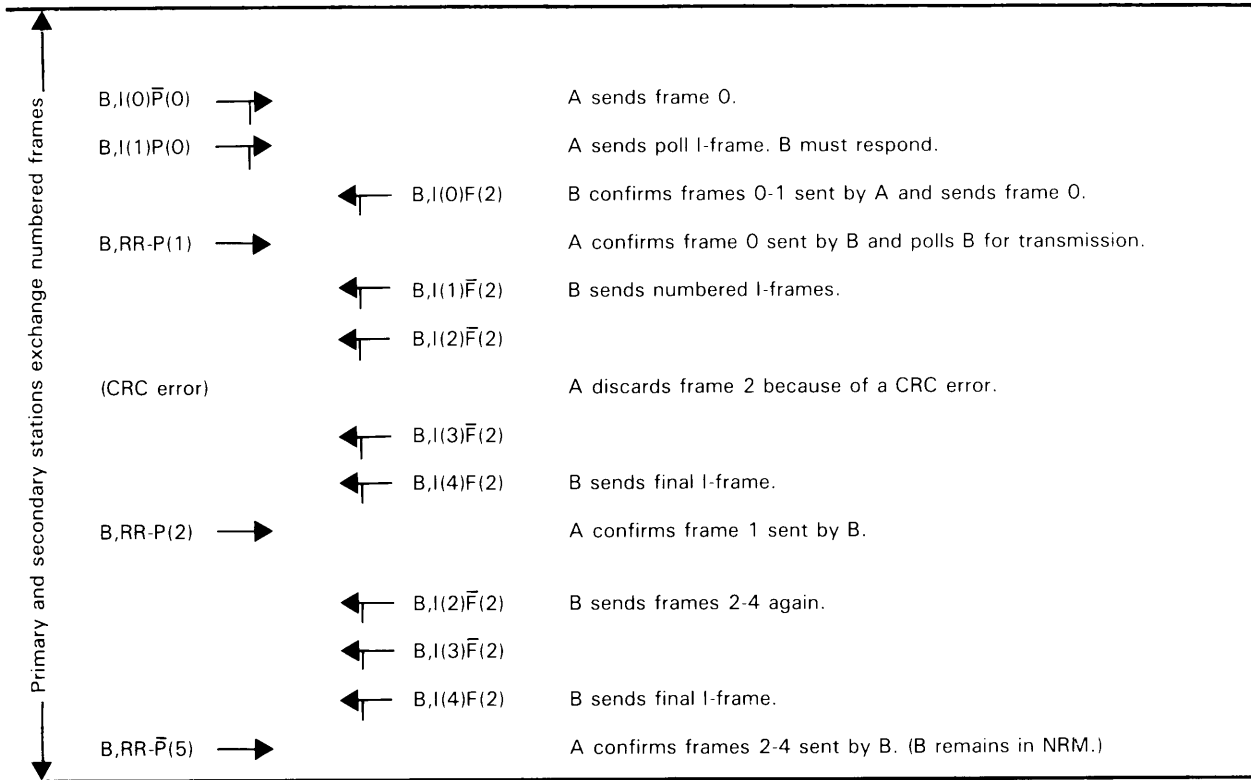
Figure 24 (Part 2 of 2). Two-way Alternate Exchanges on Nonswitched Point-to-Point Links
